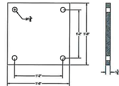
CAP AND BASE PLATE
