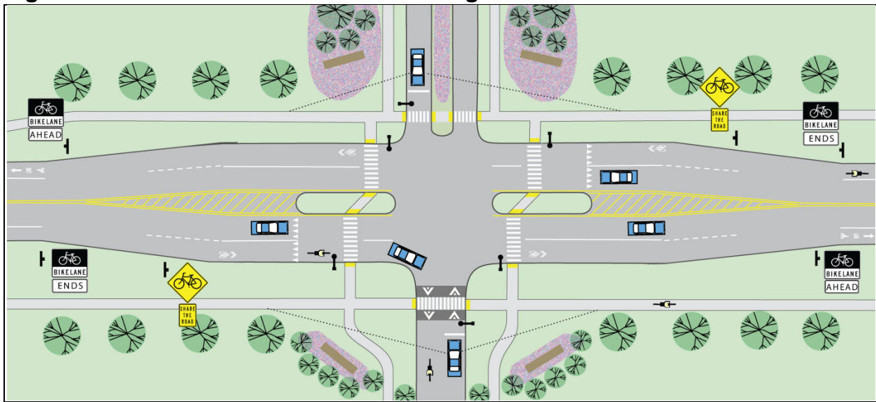
Fig. 5.4AB. Subdivision Intersection Design Guidelines
