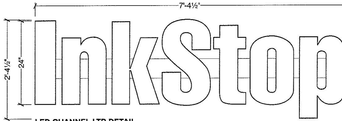
LED CHANNEL LTR DETAIL SCALE: 3/4"=1'-0" 17.51 SQ.FT
