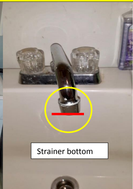
Direct Cross Connection
